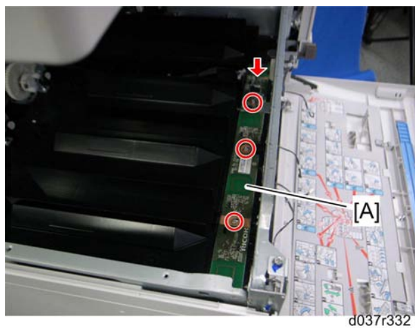
5. RFID board [A] (🔩 x 3, 📡 x 1)
