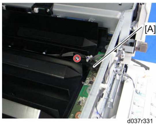
4. Harness cover [A] (🔩 x 1)
